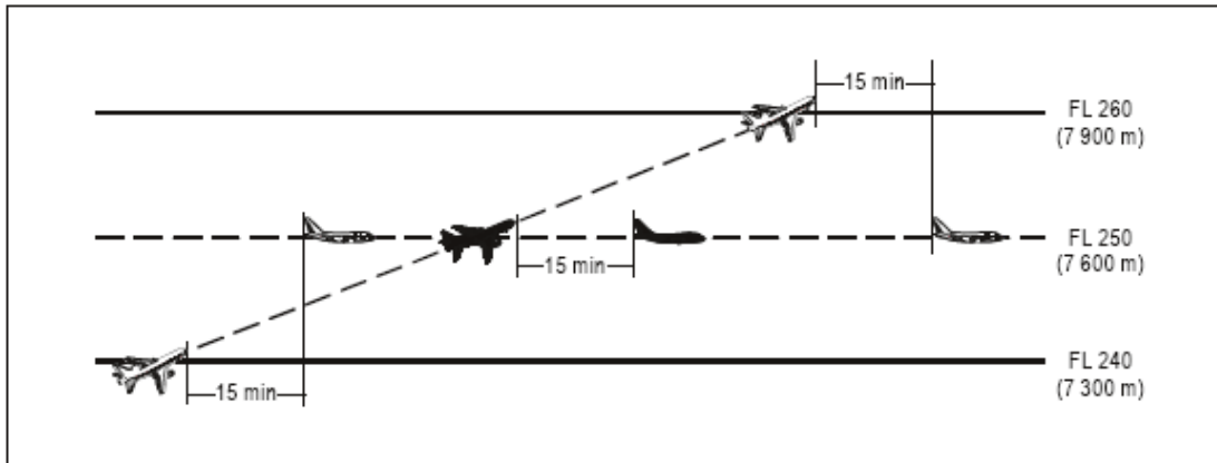
Figure 5-18A. Fifteen-minute separation between aircraft climbing and on crossing tracks (see 5.4.2.2.2.2 a))
