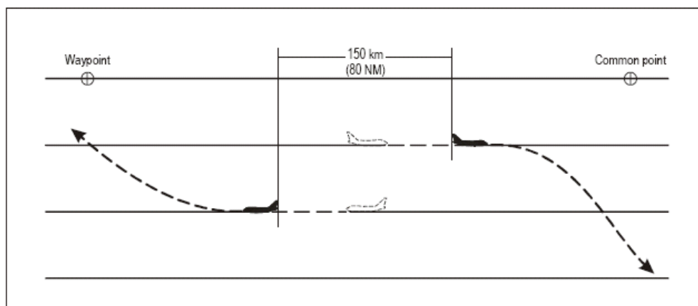
Figure 5-27. 150 km (80 NM) RNAV-based separation between aircraft on reciprocal tracks (see 5.4.2.5.7)
