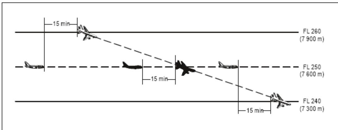
Figure 5-18B. Fifteen-minute separation between aircraft descending and on crossing tracks (see 5.4.2.2.2.2 a))
