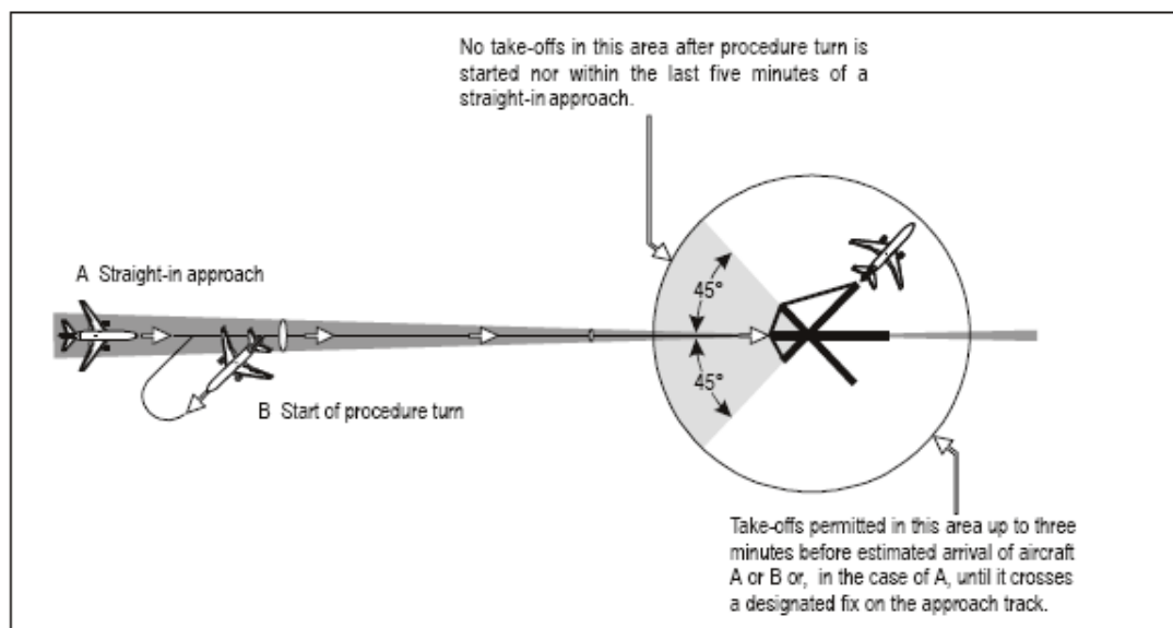
Figure 5-38. Separation of departing aircraft from arriving aircraft (see 5.7.1.1 b) and 5.7.1.2 b))
