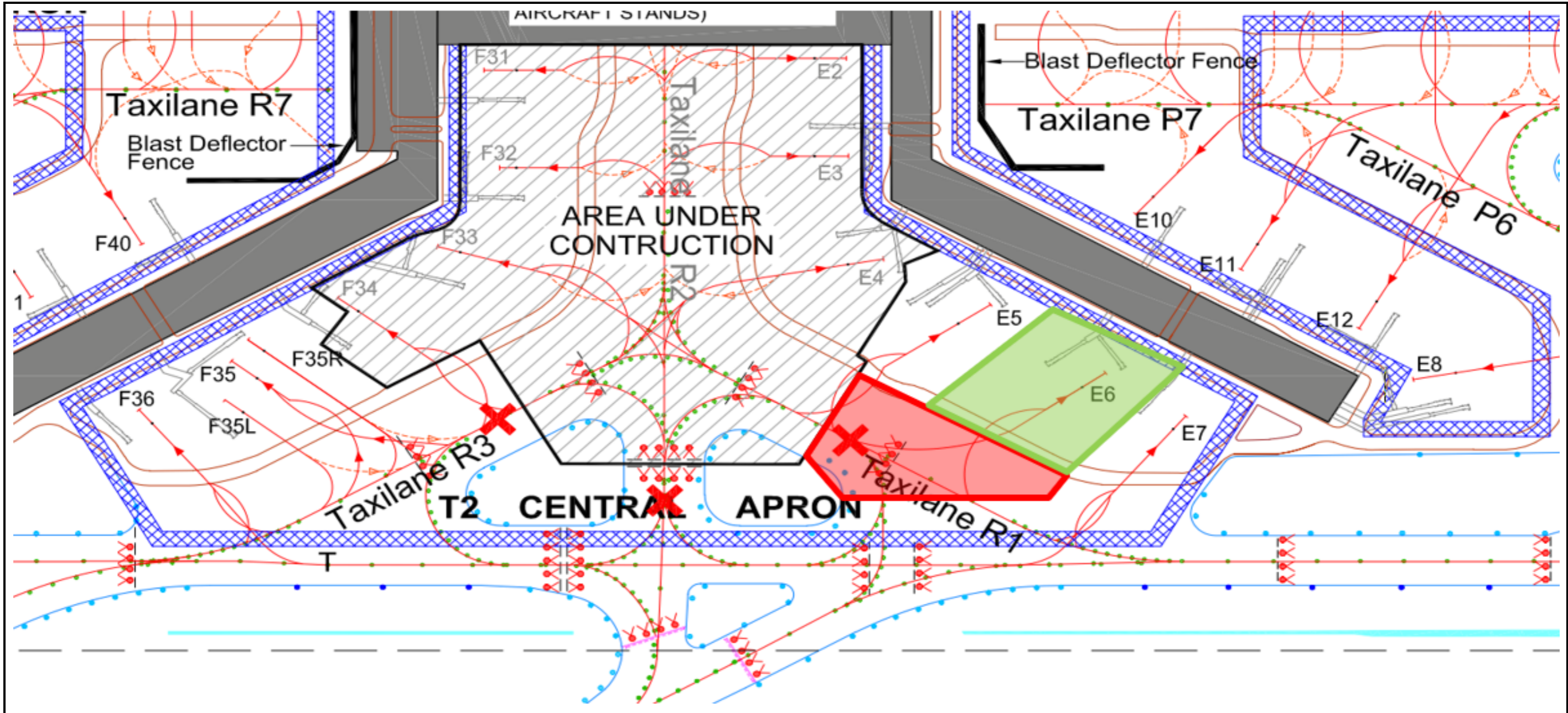
Enlarged Location Plan of Closed Section at Aircraft Stand E6 and Taxilane R1 behind Aircraft Stand E5 and E6, Singapore Changi Airport
