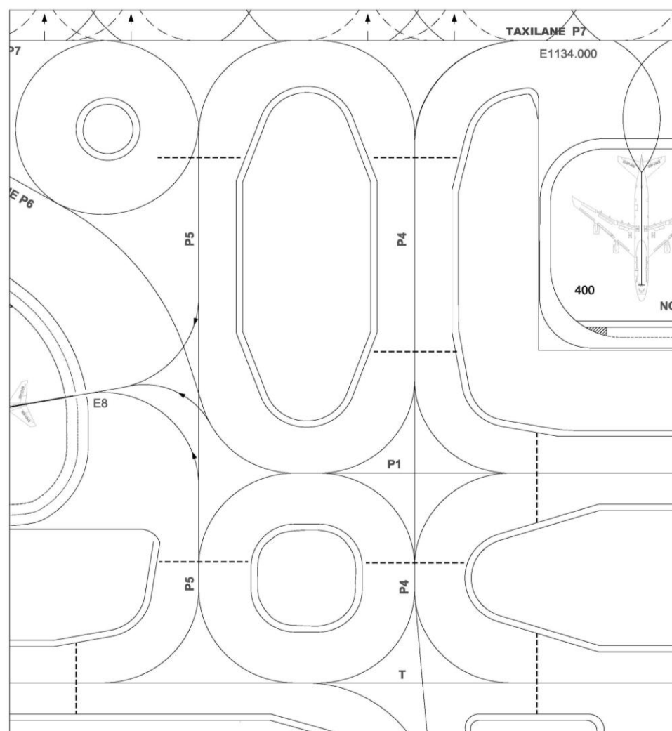
EXISTING TAXIWAY P4 MARKINGS
