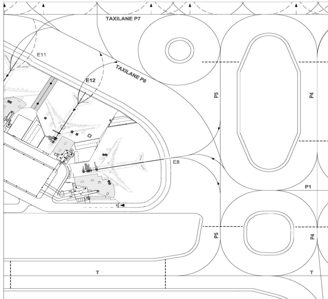
EXISTING AIRCRAFT STANDS E12 AND E8 LEAD-IN LINES, TAXIWAY P5 AND TAXILANE P6 MARKINGS
