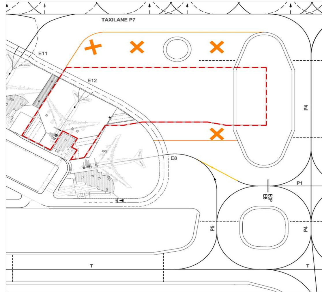
REVISION TO AIRCRAFT STANDS E12 AND E8 LEAD-IN LINES, TAXIWAY P5 AND TAXILANE P6 MARKINGS
