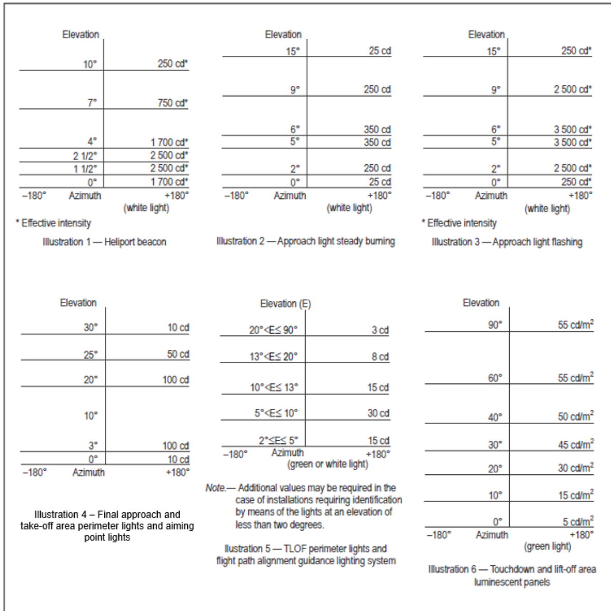
Figure 6-5. Isocandela diagrams
