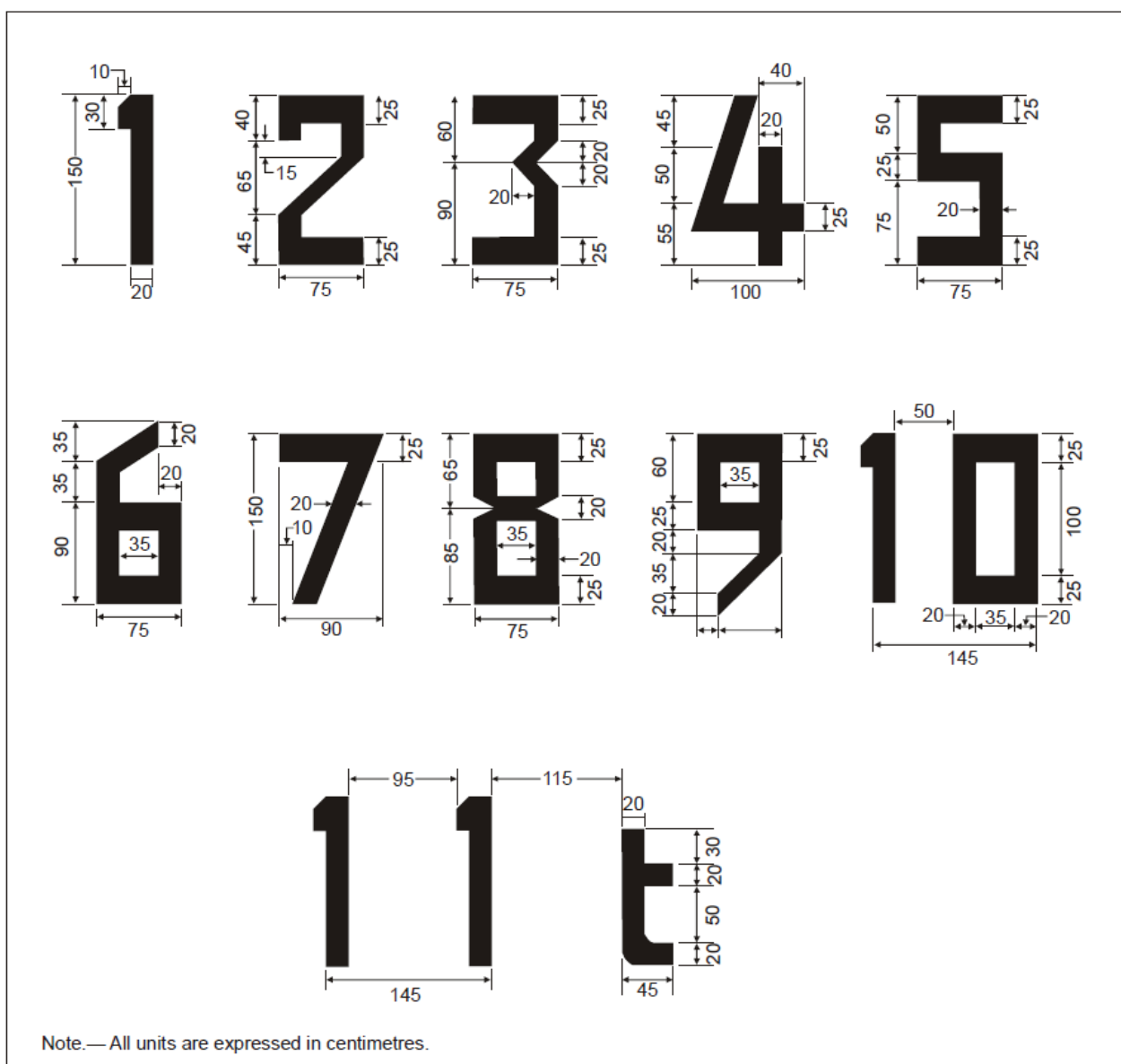
Figure 6-3 Form and proportions of numbers and letters
