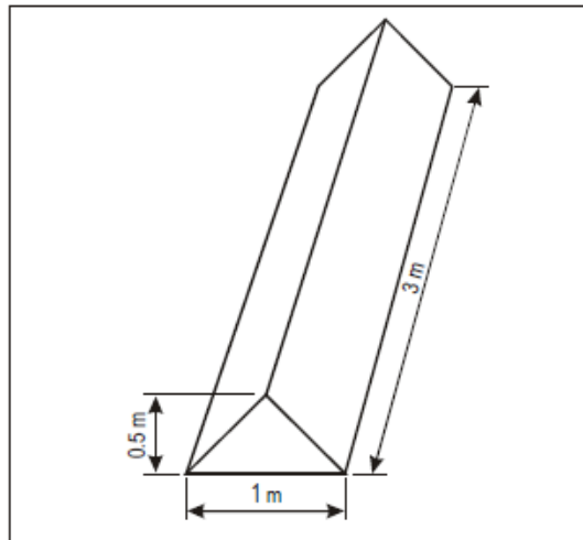
Figure 8-27. Boundary markers
