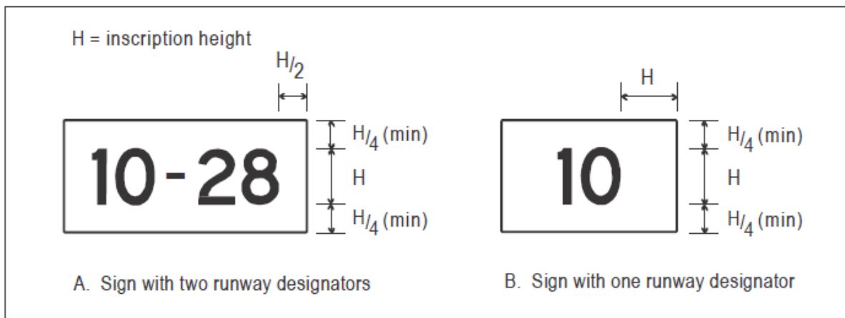
Figure A5-4. Sign dimensions
