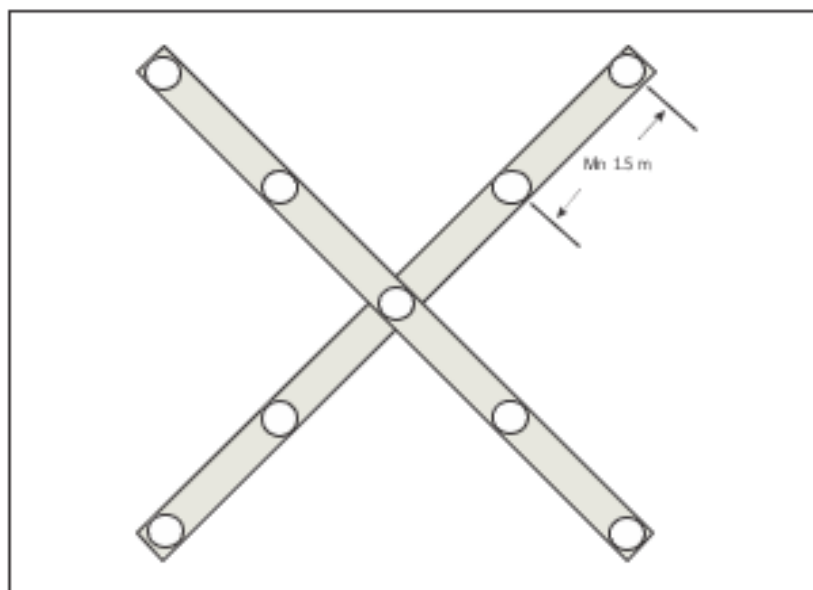
Figure 10-2A – Example of equivalent elevated closed runway lighting with five lights per branch
