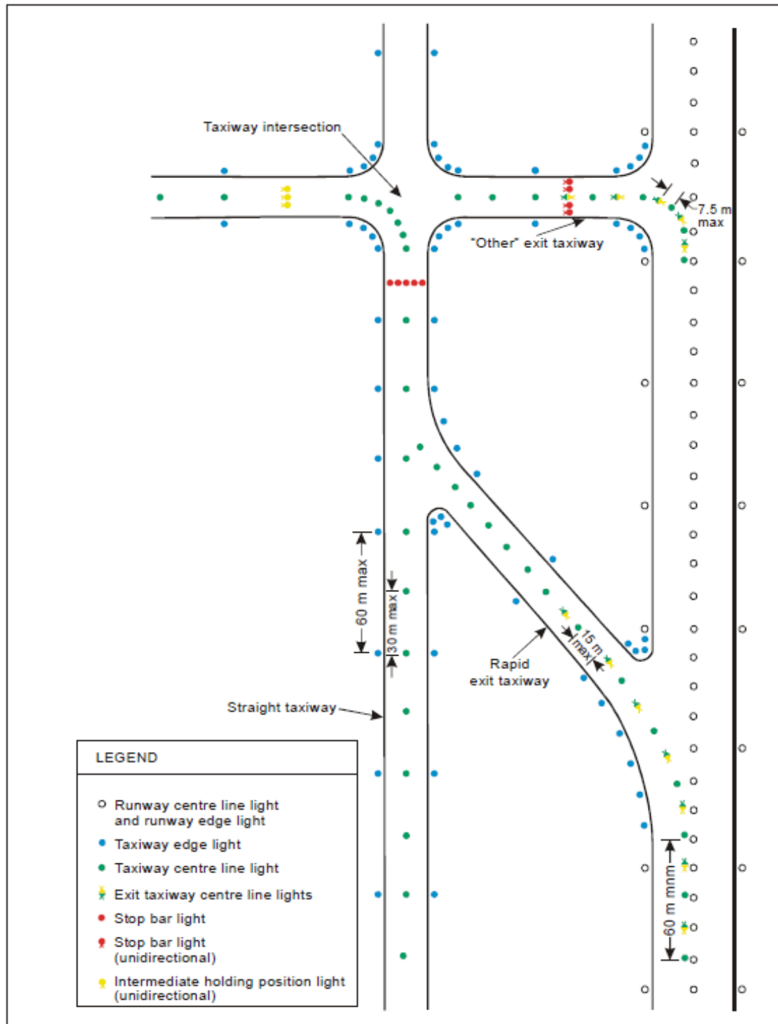
Figure 8-22. Taxiway lighting
