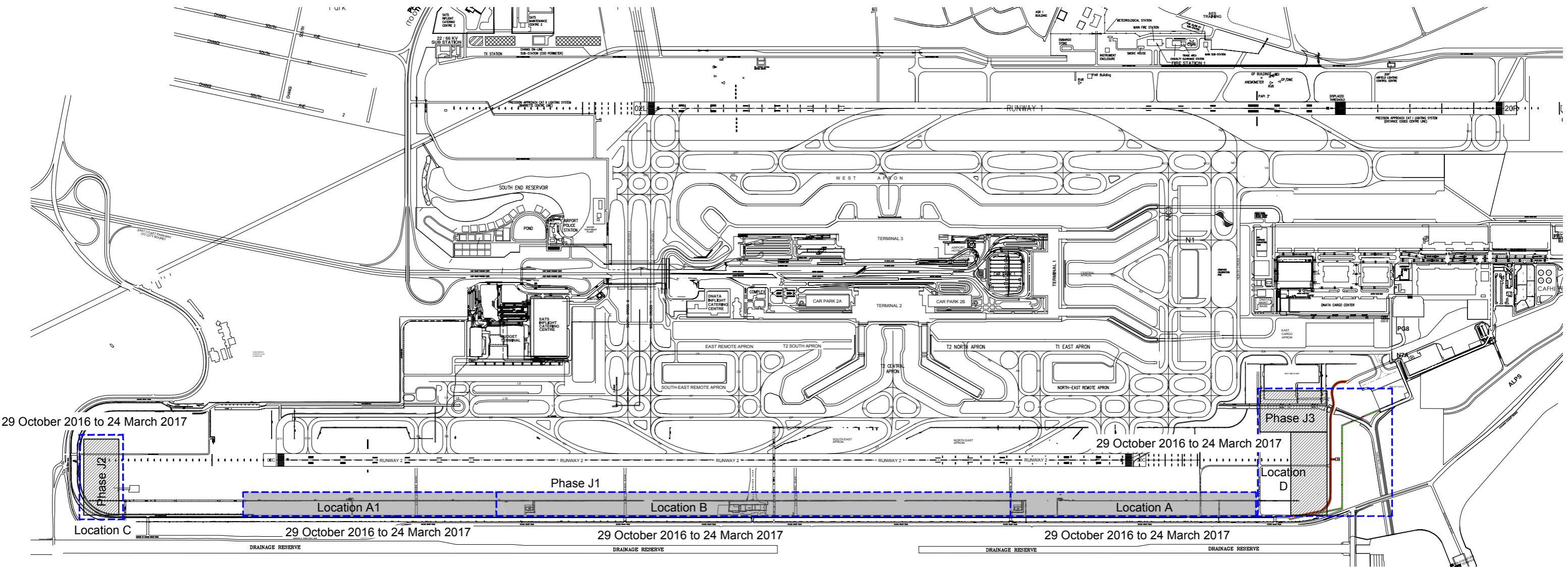
Soil Improvement Work Construction Phases and Location
