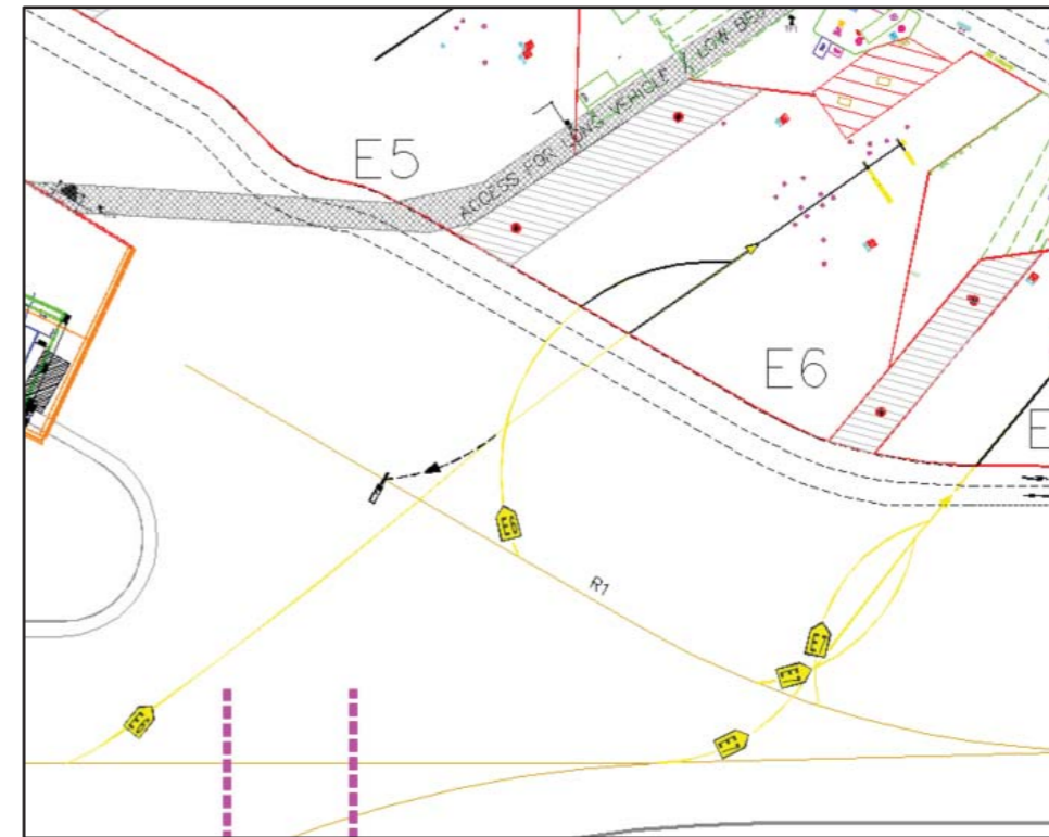
REVISION TO AIRCRAFT STAND E6 LEAD-IN LINE AND TAXIWAY/TAXILANE MARKINGS
